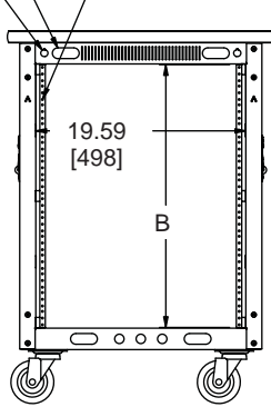
PTRK-XXMDK REAR VIEW
